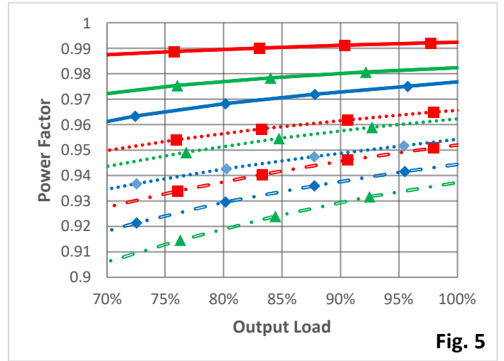
Power Factor vs. Load
