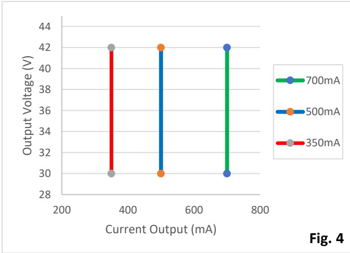
Operating Window
